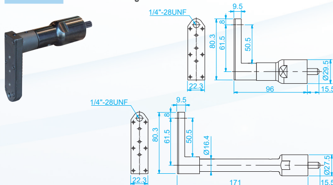
AD70H-F 114mm Offset Angle Head
