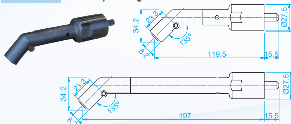
AD70H-AL 45° Compact Angle Head Extended
