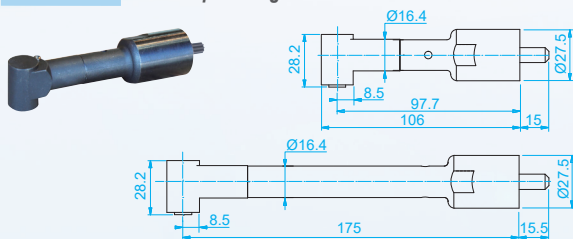
AD70H-BL 90° Compact Angle Head Extended
