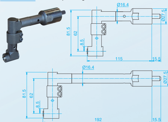
AD70H-DL 360° Compact Angle Head Extended
