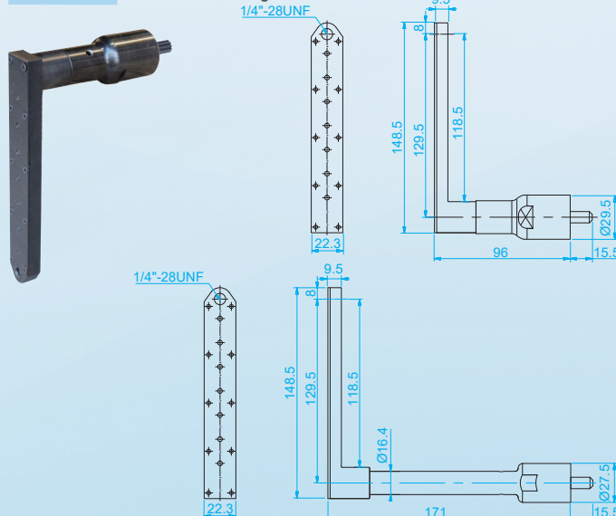
AD70H-GL 148mm Offset Angle Head Extended
