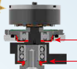
Dust Resistant Structure
