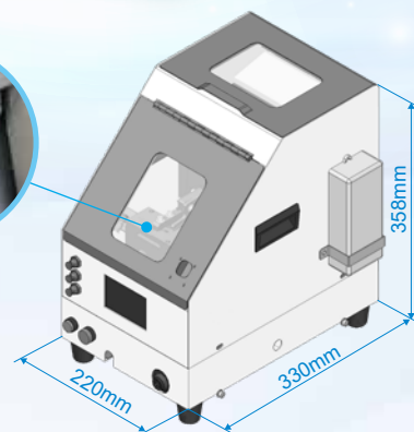
Drum-type through design
