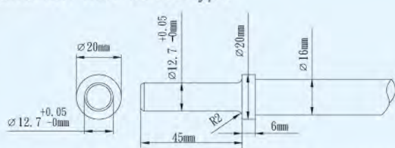
Round 12.7 mm for RC type
