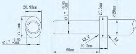
Φ20mm Round 17 mm Round Collar for RB type
