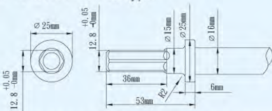
Hex. 12.8 mm for HC type
