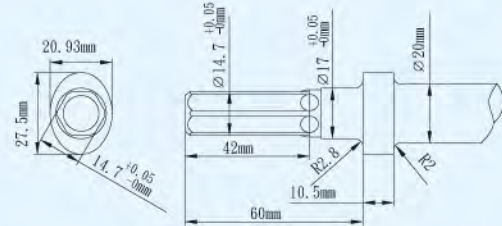
Φ20mm Hex. 14.7mm Oval Collar for HA type
