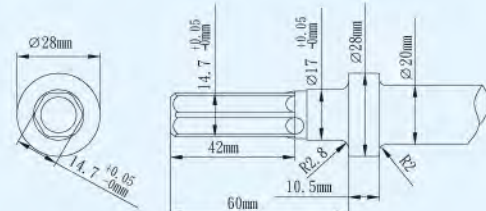
Φ20mm Hex. 14.7mm Round Collar for HB type
