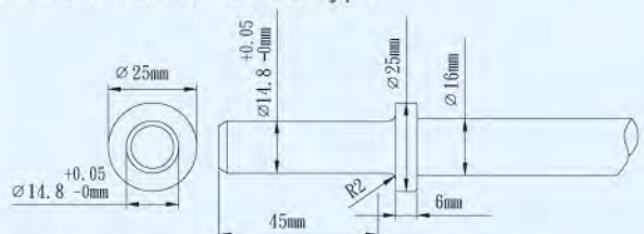
Round 14.8mm for RB type
