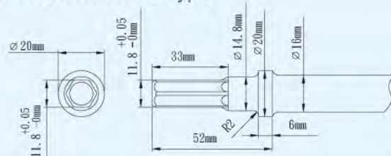
Hex. 11.8 mm for HA type
