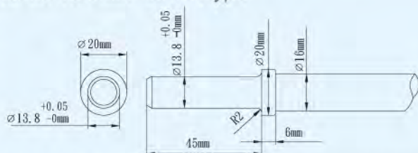
Round 13.8mm for RA type
