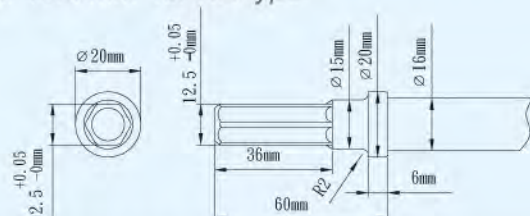
Hex. 12.5 mm for HB type
