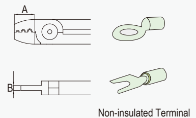
Non-insulated Terminal
