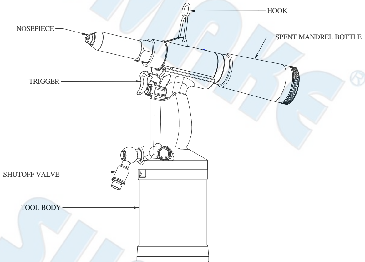
Fig. 1 UV/883; 4X Rivet-Pull Tool
