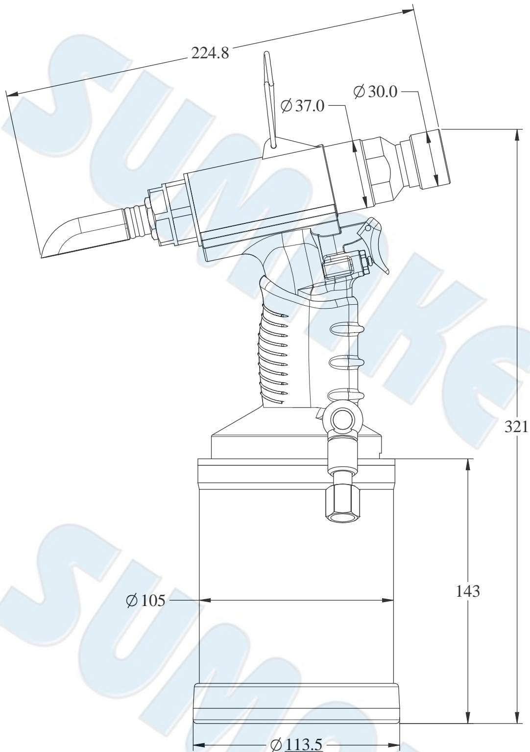
Fig.4 OUTLINE DIMENSIONS
